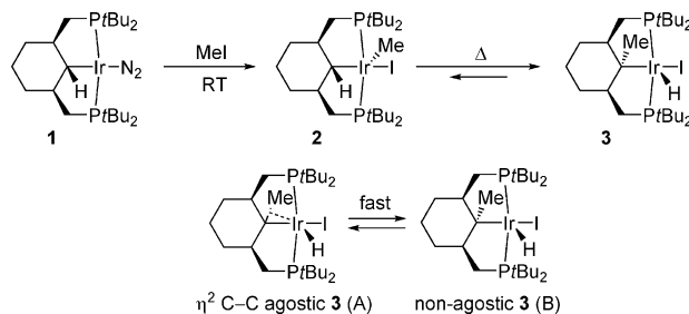
Scheme 2. Synthesis of 2 and subsequent transformation into compound 3 .
